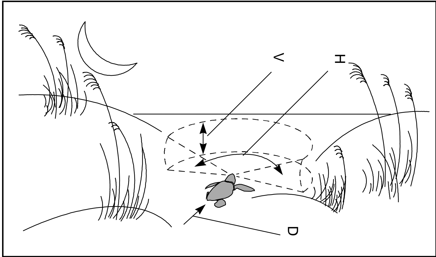
Figure 2. A hypothetical cone of acceptance that describes how a sea turtle hatchling measures brightest direction. The vertical component of the cone (V) is approximately 10-30^\circ from the horizon, and the horizontal component of the cone (H) is approximately 180^\circ . Light sources within this cone of acceptance are thought to be integrated into an assessment of brightness for the direction D. Figure taken from Witherington, 1997, with permission.
